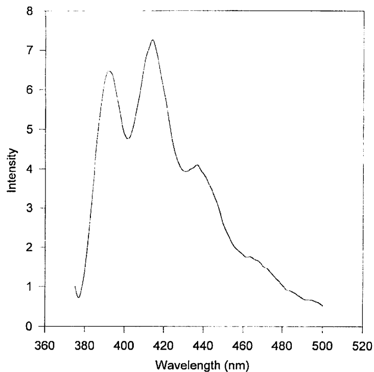
Figure 4.8. Fluorescence spectrum of \text{PDA}^+\text{SbF}_6^- at room temperature.
