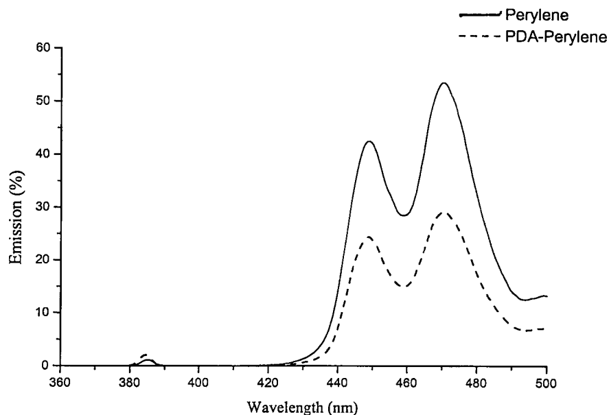
Figure 4.5. Quenching of perylene fluorescence emission at \lambda_{\text{ex}}=386 nm by \text{PDA}^+\text{SbF}_6^- in \text{CH}_2\text{Cl}_2 , [\text{PDA}]=1 \times 10^{-4} mol \text{L}^{-1} , [\text{perylene}]=1 \times 10^{-4} mol \text{L}^{-1}
