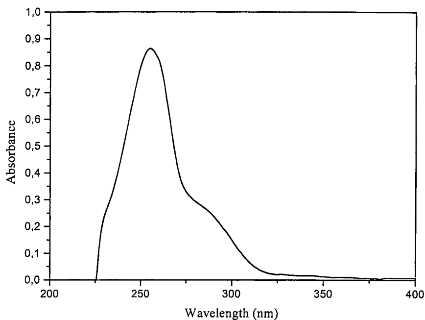
Figure 4.1. Absorption spectrum of \text{PDA}^+\text{SbF}_6^- ( 4 \times 10^{-5} \text{ mol l}^{-1} ) in \text{CH}_2\text{Cl}_2
