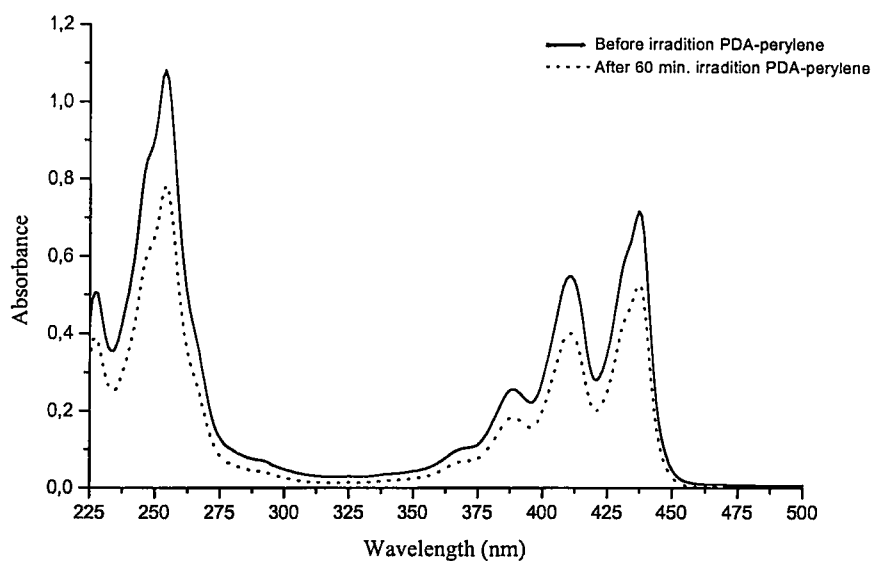
Figure 4.7. Absorption spectra of \text{PDA}^+\text{SbF}_6^- ( 8 \times 10^{-6} \text{ mol L}^{-1} ) and perylene ( 8 \times 10^{-6} \text{ mol L}^{-1} ) in \text{CH}_2\text{Cl}_2 before (—) and after 60 min. irradiation (···) at \lambda = 440 \text{ nm}
