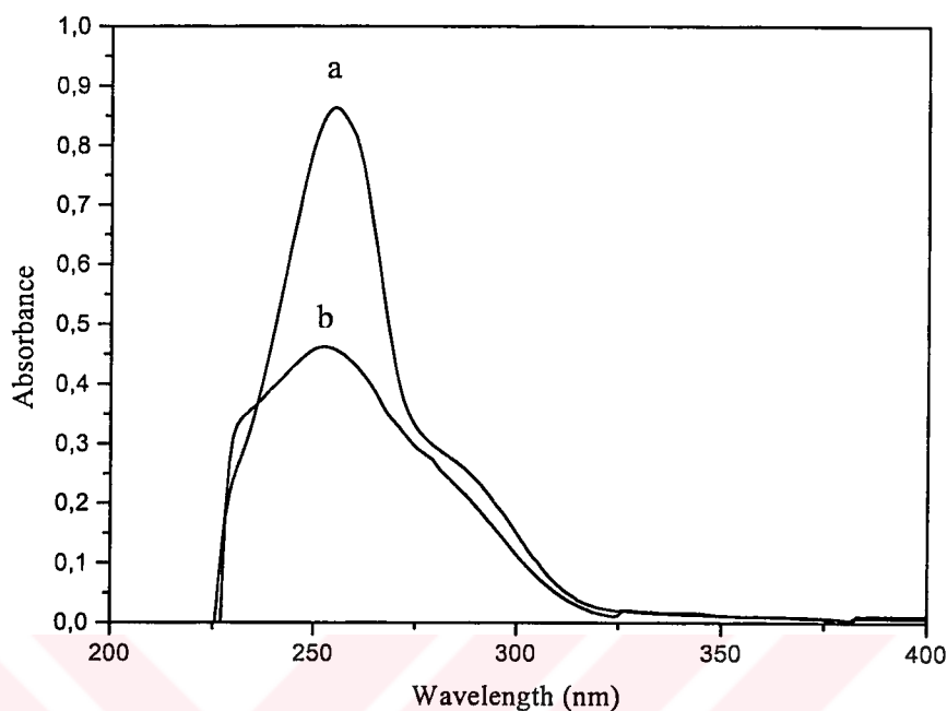
Figure 4.3. Absorption spectra of \text{PDA}^+\text{SbF}_6^- ( 4 \times 10^{-5} \text{ mol L}^{-1} ) in \text{CH}_2\text{Cl}_2 before (a) and after 15 min irradiation (b).
