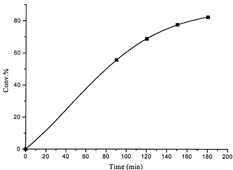
Figure 4.2. Photopolymerization of CHO by using \text{PDA}^+\text{SbF}_6^- at \lambda > 300 nm. [\text{PDA}^+\text{SbF}_6^-] = 5 \times 10^{-3} \text{ M}
