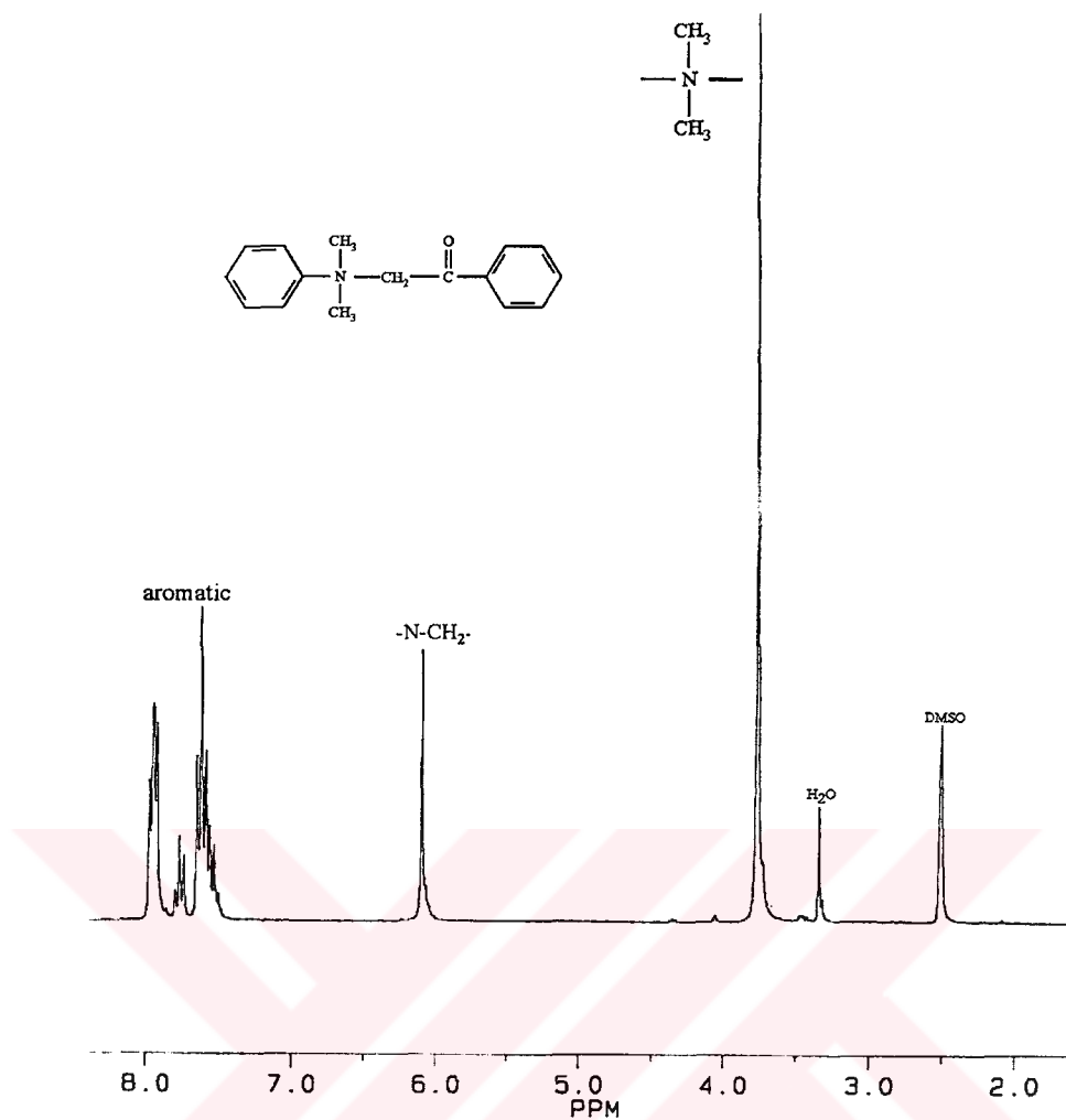
Figure 3.1. ^1\text{H-NMR} spectrum of N -phenacyl N,N -dimethylanilinium hexafluoroantimonate in DMSO
