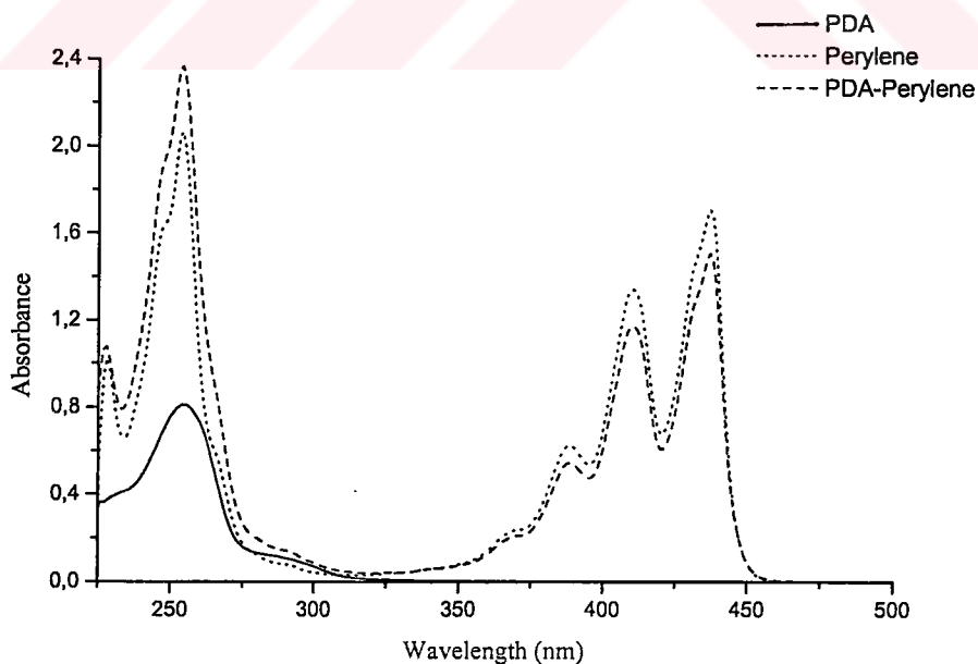
Figure 4.6. Absorption spectra of \text{PDA}^+\text{SbF}_6^- , perylene, \text{PDA}^+\text{SbF}_6^- +perylene ( 4 \times 10^{-5} mol \text{L}^{-1} ) in \text{CH}_2\text{Cl}_2 solution
