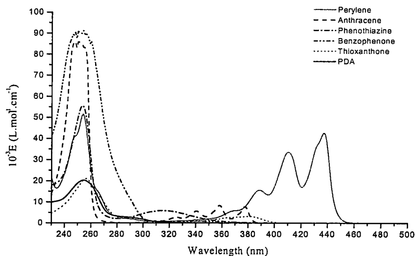
Figure 4.4. Optical absorption spectra of perylene, anthracene, phenothiazine, benzophenone, thioxanthone and \text{PDA}^+\text{SbF}_6^- in \text{CH}_2\text{Cl}_2 solution
