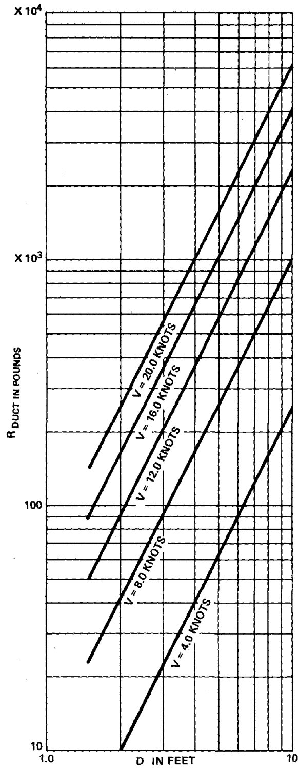
Figure 8 - Relationship for Estimating the Resistance of Well-Faired Duct Openings
