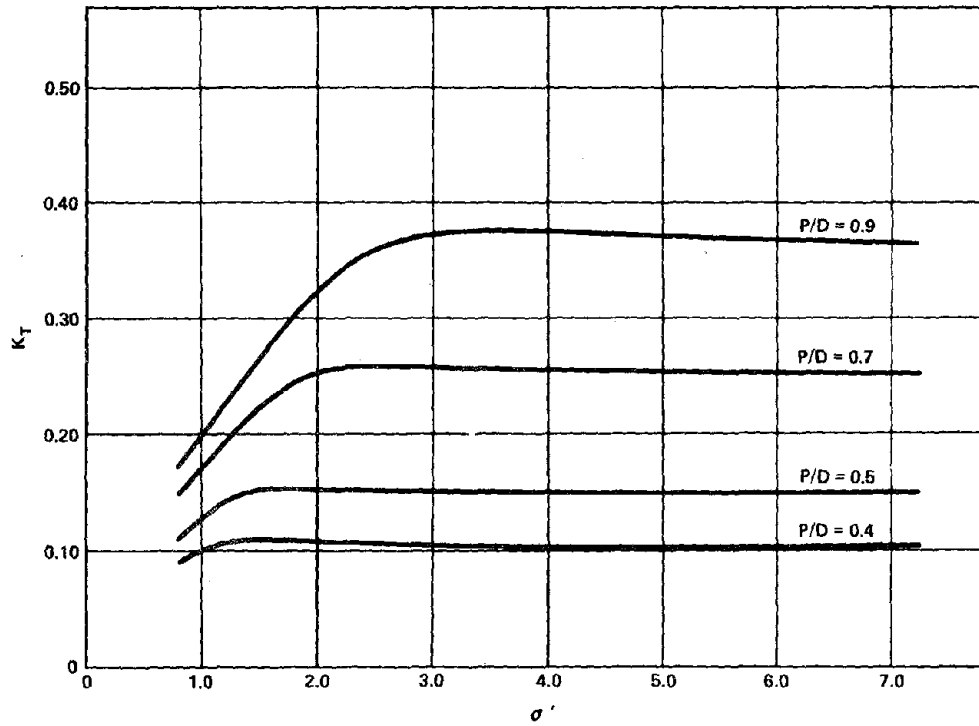
Figure 12a - Thrust Coefficient
