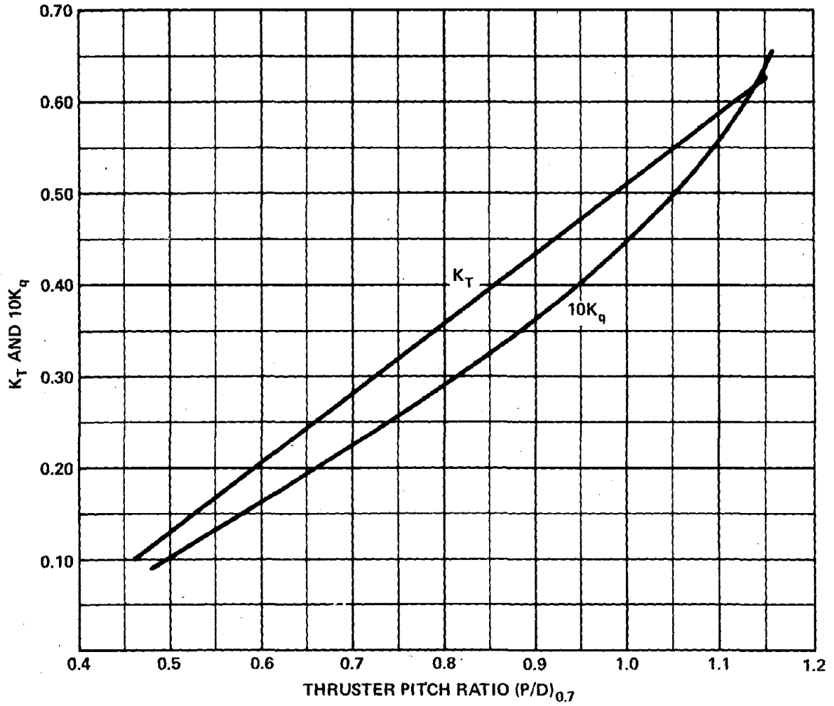
Figure 11 - K_T and K_Q versus Pitch Ratio for DSRV Bow Thruster with NSRDC Adjustable-Pitch Propeller 4160
