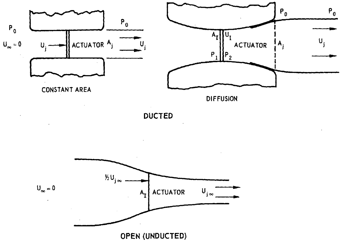
Figure 1 - Idealized Flow for Ducted and Open-Type Thrusters
