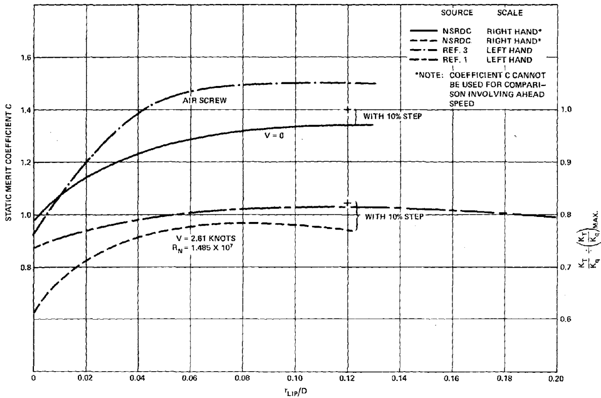
Figure 7 - Criteria for Establishing Duct Lip Radius
