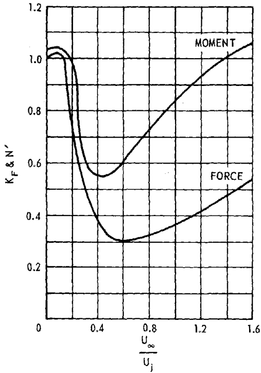
Figure 2b - Surface Ship (According to Reference 2.)
