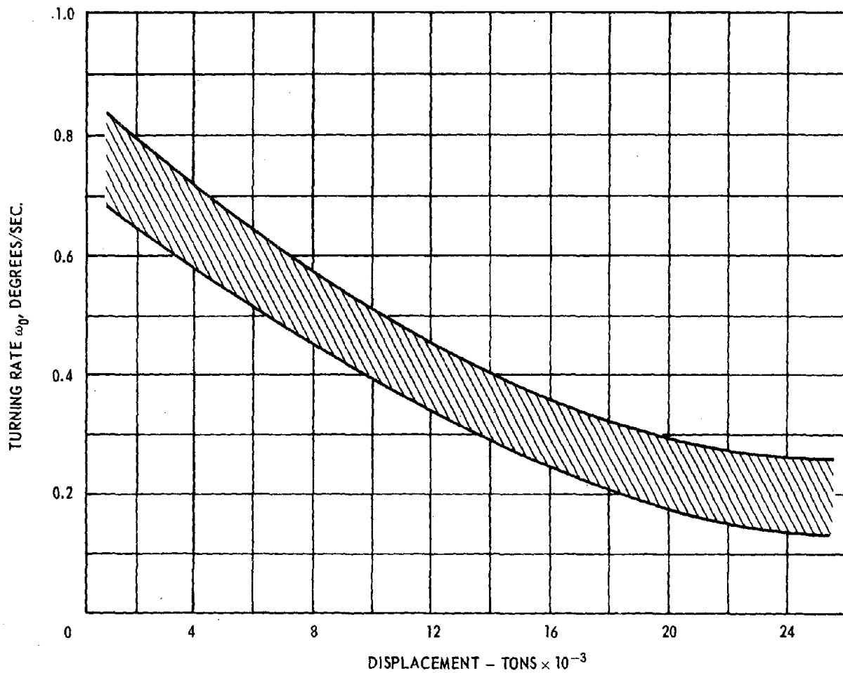
Figure 3 - Band of Rotation Rates versus Displacement with MPD at Zero Ship Speed (according to Reference 6)
