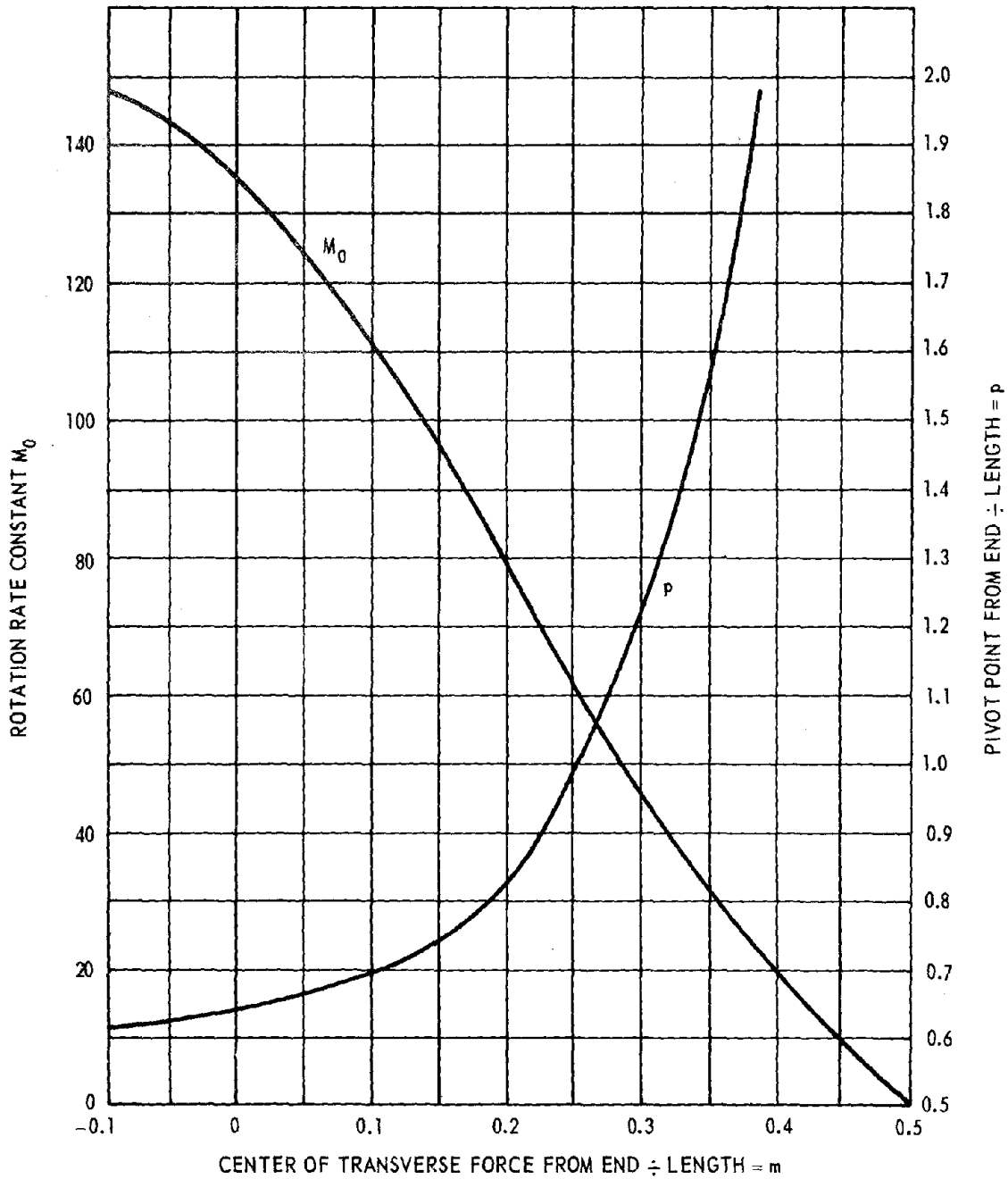
Figure 4 - Pivot Point and Rotation Rate Constant for a Single Side Force Acting on a Ship (according to Reference 6)
