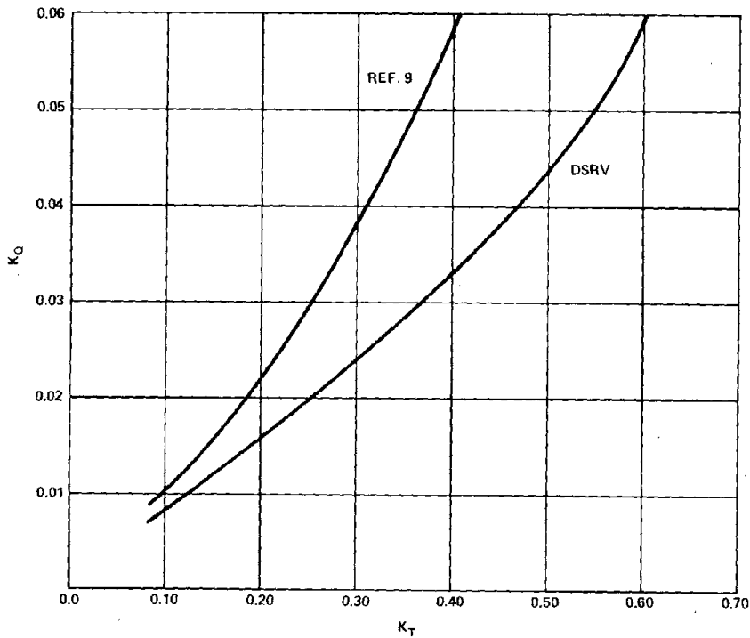
Figure 10 - K_Q versus K_T Obtained at Discrete Pitch Ratios for Adjustable Pitch Propellers (Noncavitating), V = 0
