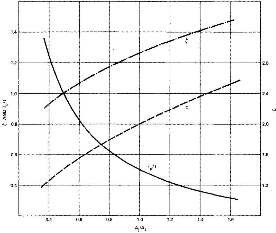
Figure 6 - Idealized Variation of \zeta , C and T_p/T with Exit Area Ratio
