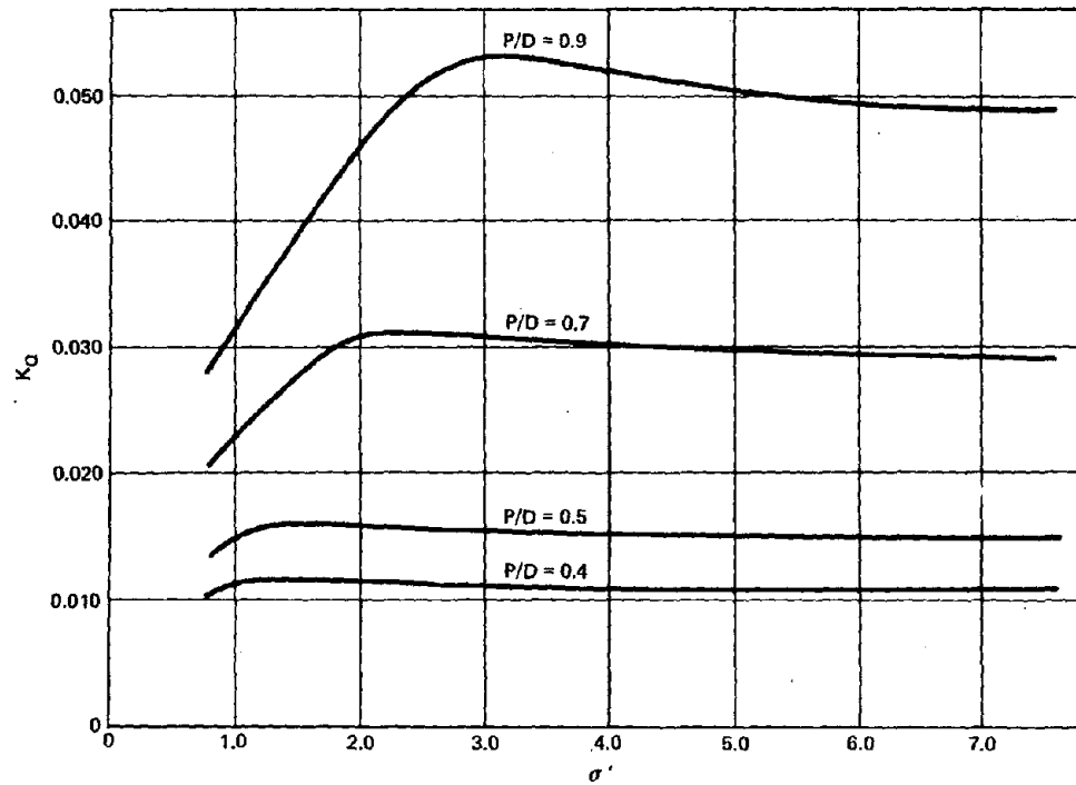
Figure 12b - Torque Coefficient
