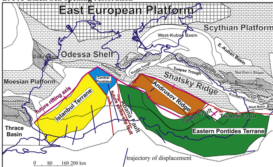
Figure 11. Pre-Black Sea Basin Opening Tectonic Structure Restoration. Figure A shows possible outlines of gaps in the restoration (see discussion in the text). Figure B shows the tectonic structure before the Black Sea Basin opening. Arrows show trajectories of displacements during the Black Sea Basin opening.
