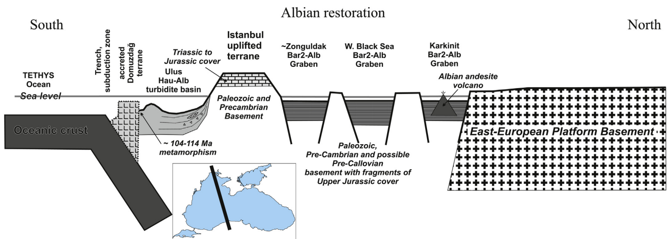
Figure 7. Albian Structure Restoration, Western Black Sea Basin. Data on metamorphism are from Okay et al. (2013). Hau – Hauterivian, Alb – Albian, Bar – Barremian.
