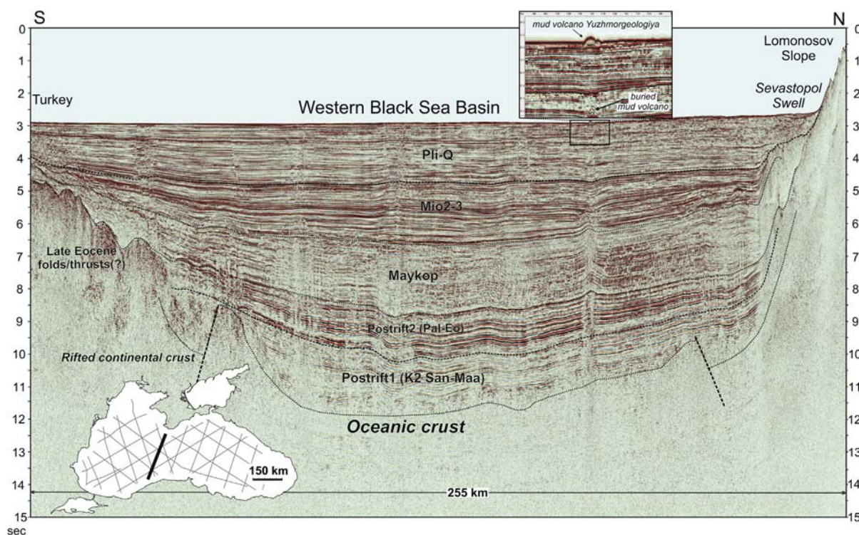
Figure 20. Geological interpretation of seismic line BS-260. This line shows some structure of the Western Black Sea Basin. The Sevastopol Swell possibly corresponds to a transpressional structure. A recent, active mud volcano is recognized as a positive structure on the sea bed; at depth, a buried mud volcano system is seen, with roots in the Maykopian stratigraphic level.
