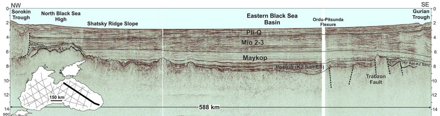
Figure 14. Geological interpretation of seismic line BS-180. This line follows the axis of the Eastern Black Sea Basin. The North Black Sea High, one of the highest uplifts of the Shatsky Ridge, was a tilted block during Maykopian times and acted as a peripheral bulge simultaneously for the Sorokin and Tuapse foredeep flexural basins. The Ordu–Pitsunda Flexure separates the Eastern Black Sea and the Trabzon basins. The Gurian Trough has no anomalously thick Maykopian deposits as compared with the Tuapse and Sorokin troughs. The Gurian Trough is possibly Miocene in age and it is not analogous to the Tuapse and Sorokin troughs.
