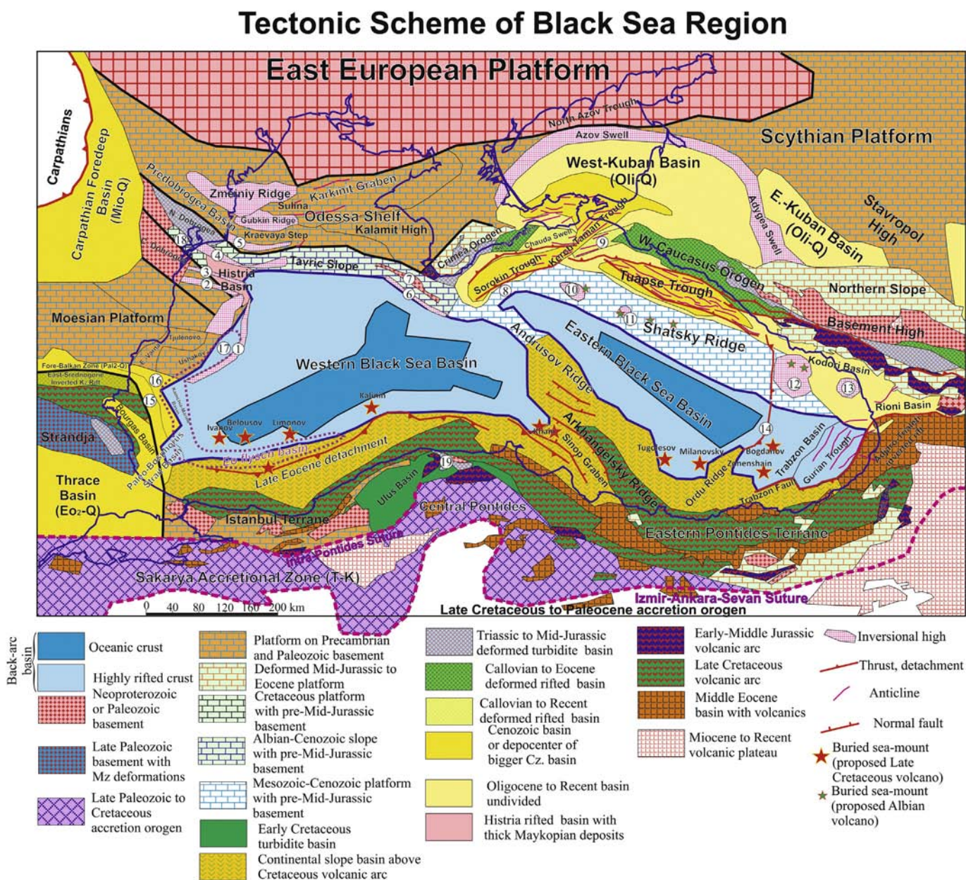
Figure 1. Tectonic map of the Black Sea region. The map is compiled by using both new data presented in this paper and published data (Tugolev et al., 1985; Okay et al., 1994, 2013; Robinson et al., 1996; Afanasev et al., 2007; Khriachtchevskaya et al., 2010; Munteanu et al., 2011; Nikishin et al., 2012; Georgiev, 2012). Eo – Eocene, T-K – Triassic to Cretaceous. 1 – Polshkov Ridge, 2 – Tindala-Midia Ridge, 3 – Tomis Ridge, 4 – Lebada Ridge, 5 – Sf. Georg Ridge, 6 – Sevastopol Swell, 7 – Lomonosov Massif, 8 – Tetyaev Ridge, 9 – Anapa Swell, 10 – North Black Sea High, 11 – South-Doobskaya High, 12 – Gudauta High, 13 – Ochamchira High, 14 – Ordu–Pitsunda Flexure, 15 – Rezovo-Limankoy Folds, 16 – Kamchia Basin, 17 – East-Moesian Trough, 18 – Babadag Basin, 19 – Küre Basin.
