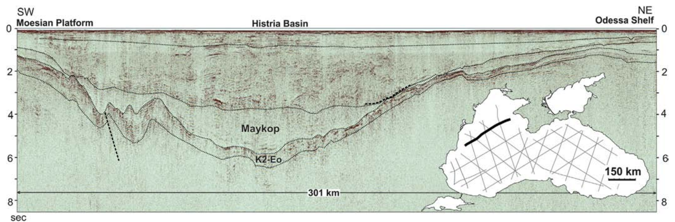
Figure 19. Geological interpretation of seismic line BS-240. This line shows the structure of the Hystria Basin, which was effected by inversion tectonics during the Late Eocene to Oligocene. It was rapidly filled by Maykopian to Recent deposits.
