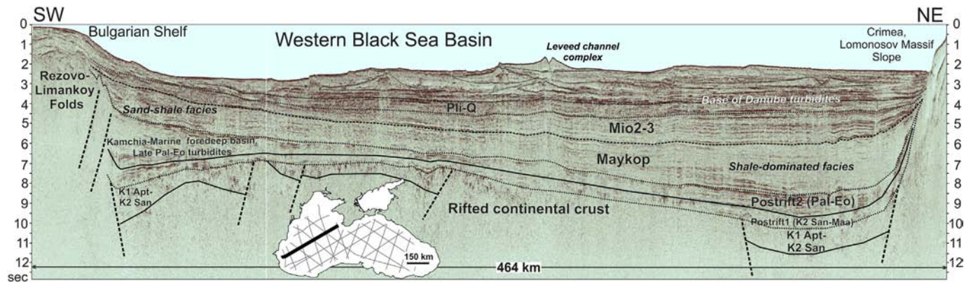
Figure 18. Geological interpretation of seismic line BS-230. Some graben-like structures are seen below the post-rift regional cover. A large sedimentary wedge of approximately Paleocene–Eocene age (pre-Maykopian) is seen close to the Bulgarian Shelf; it is interpreted as a flexural foredeep basin. This basin is probably the offshore continuation of the Kamchia Foredeep Basin of Late Paleocene–Middle Eocene age, well described in Bulgaria (Tari et al., 2009; Stuart et al., 2011; Georgiev, 2012). Large leveed channel complexes are seen between the Bulgarian and the Crimea continental slopes. The base of this complex lies close to Miocene/Pliocene boundary; according to the interpretation of this seismic line, the origin of the Danube Delta is close to the Messinian erosion event.
