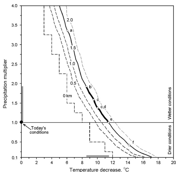
Fig. 4. Modeled length of the Kartal Lake Valley glacier (solid line) as a function of temperature and precipitation changes from those of today (full circle). As a comparison 0 km line which represents glacier inception and 0.5, 1 and 2 km lines shown (dashed lines). Thick solid and corresponding horizontal and vertical gray lines are suggested possible ranges of temperature and precipitation changes during LGM. Empty circles are those conditions suggested by proxy data (a: Bar-Matthews et al., 1997, b: Hughes et al., 2003, c: Emeis et al., 1998, 2000; Kallel et al., 2000, d: McGarry et al., 2004, e: corresponds to threshold temperature depression to sustain glacier by same amount of moisture level as today (proposed by this study), f: Jones et al., 2007).
