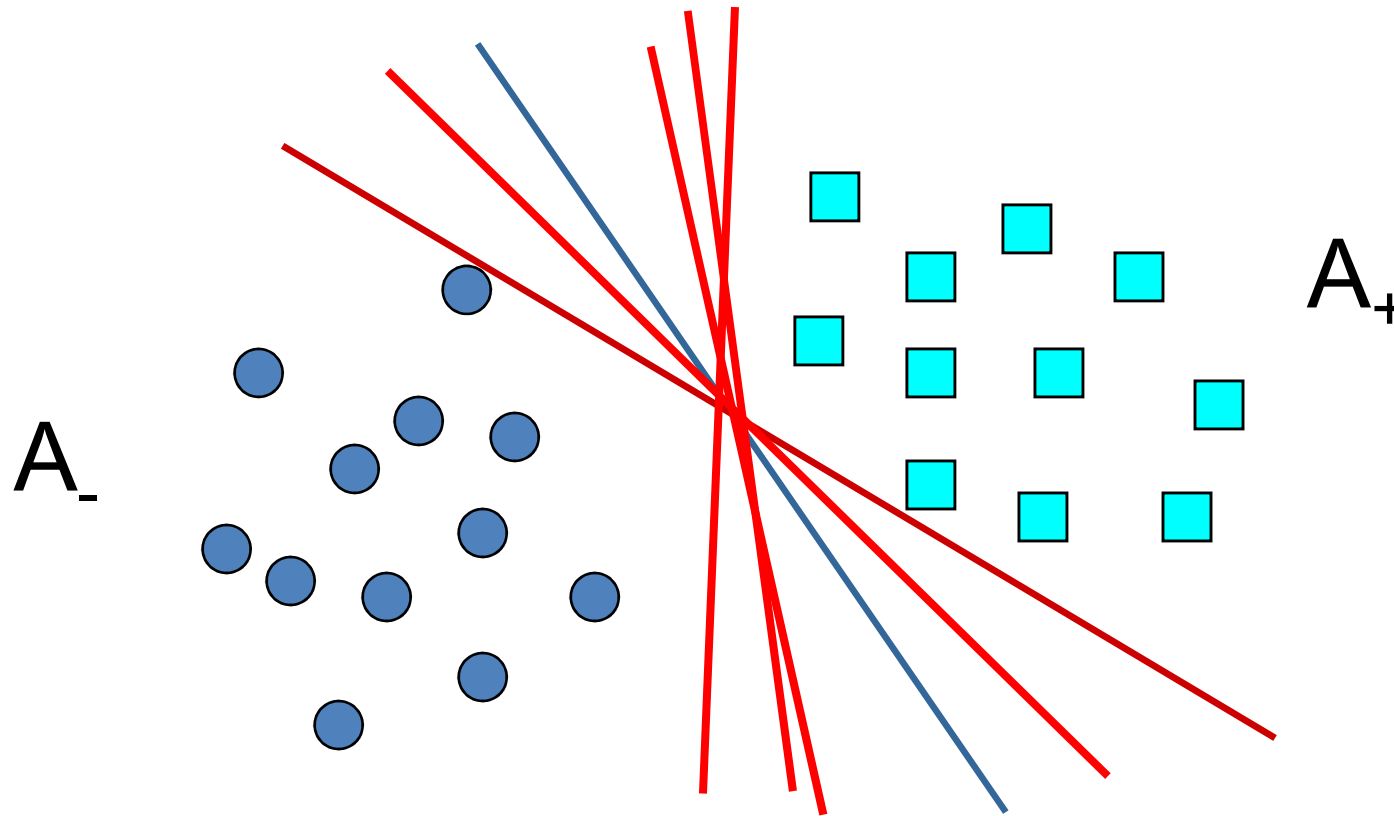
Fig. x. Linear Classification
