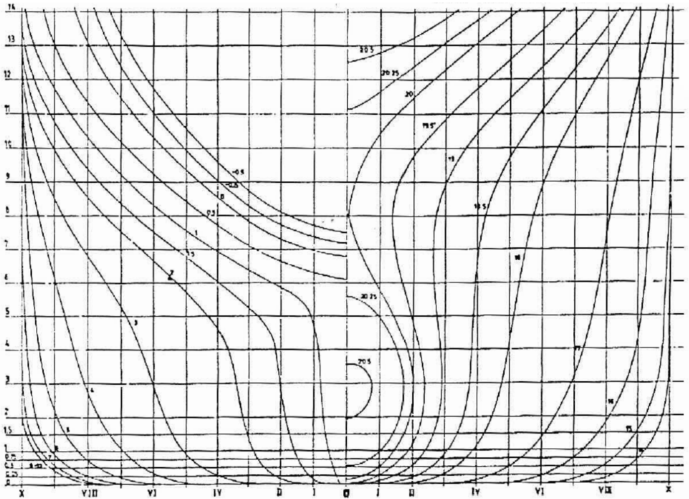
Fig. 5 Standardised sections and waterlines spacing.
