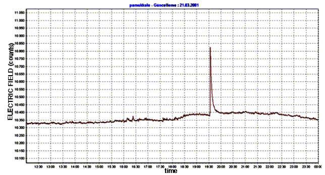
Figure 5. 37 hours before the Earthquake in Afyon Mb4.8 (March 21 st , 2001).
