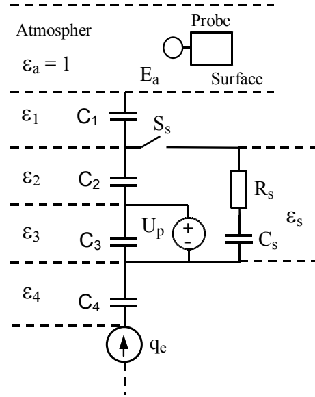
Figure 3. Equivalent circuit model of dilatency.
