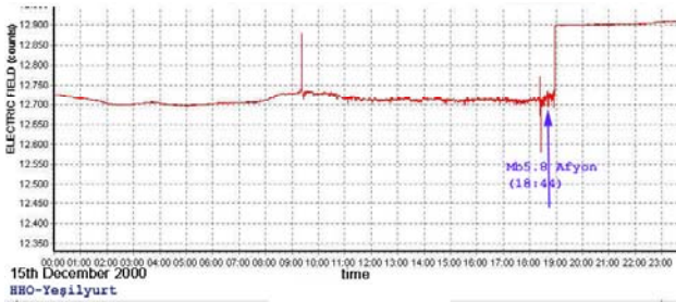
Figure 7. An example for a probable stress weakening process prior to the earthquake in Afyon Mb5.8 (December 15 th , 2000).
