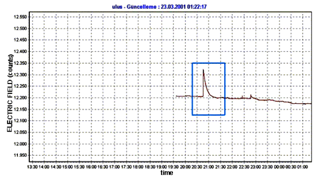
Figure 6. 40 hours before the Earthquake in Istanbul Mb3.9 (March 23 rd , 2001).
