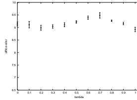
Fig. 4. The effect of increasing lambda
