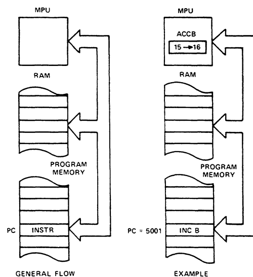
FIGURE 28 — ACCUMULATOR ADDRESSING
