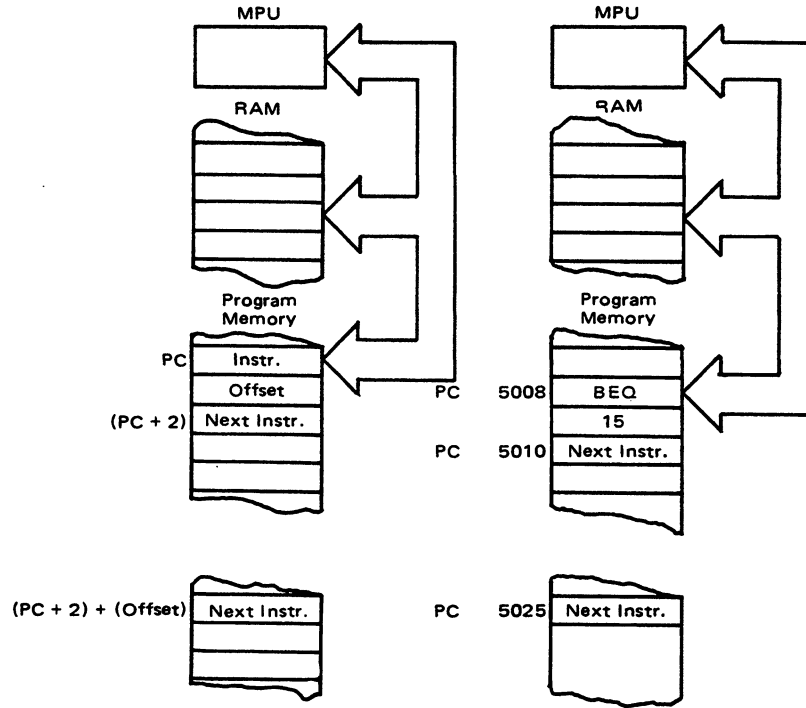
FIGURE 32 — RELATIVE ADDRESSING MODE
