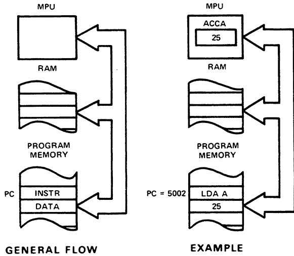
FIGURE 29 — IMMEDIATE ADDRESSING MODE
