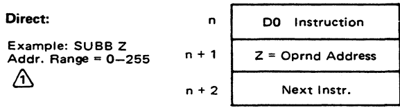
FIGURE 26 — ADDRESSING MODE SUMMARY
