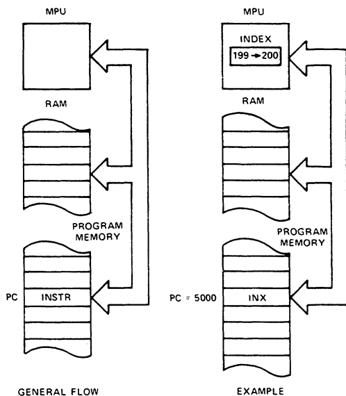
FIGURE 27 — INHERENT ADDRESSING
