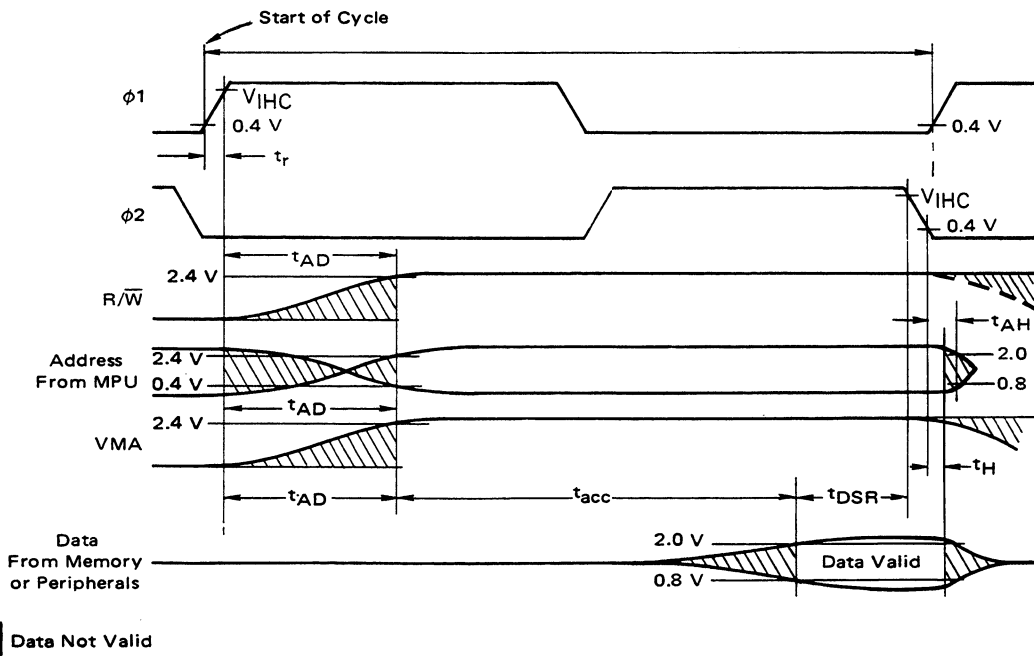
FIGURE 2 — READ DATA FROM MEMORY OR PERIPHERALS
