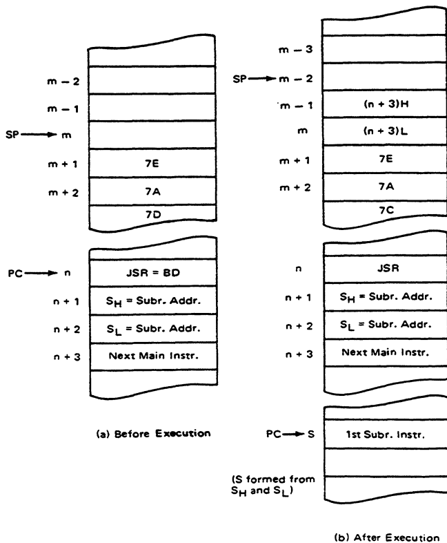
FIGURE 19 -- PROGRAM FLOW FOR JSR (EXTENDED)
