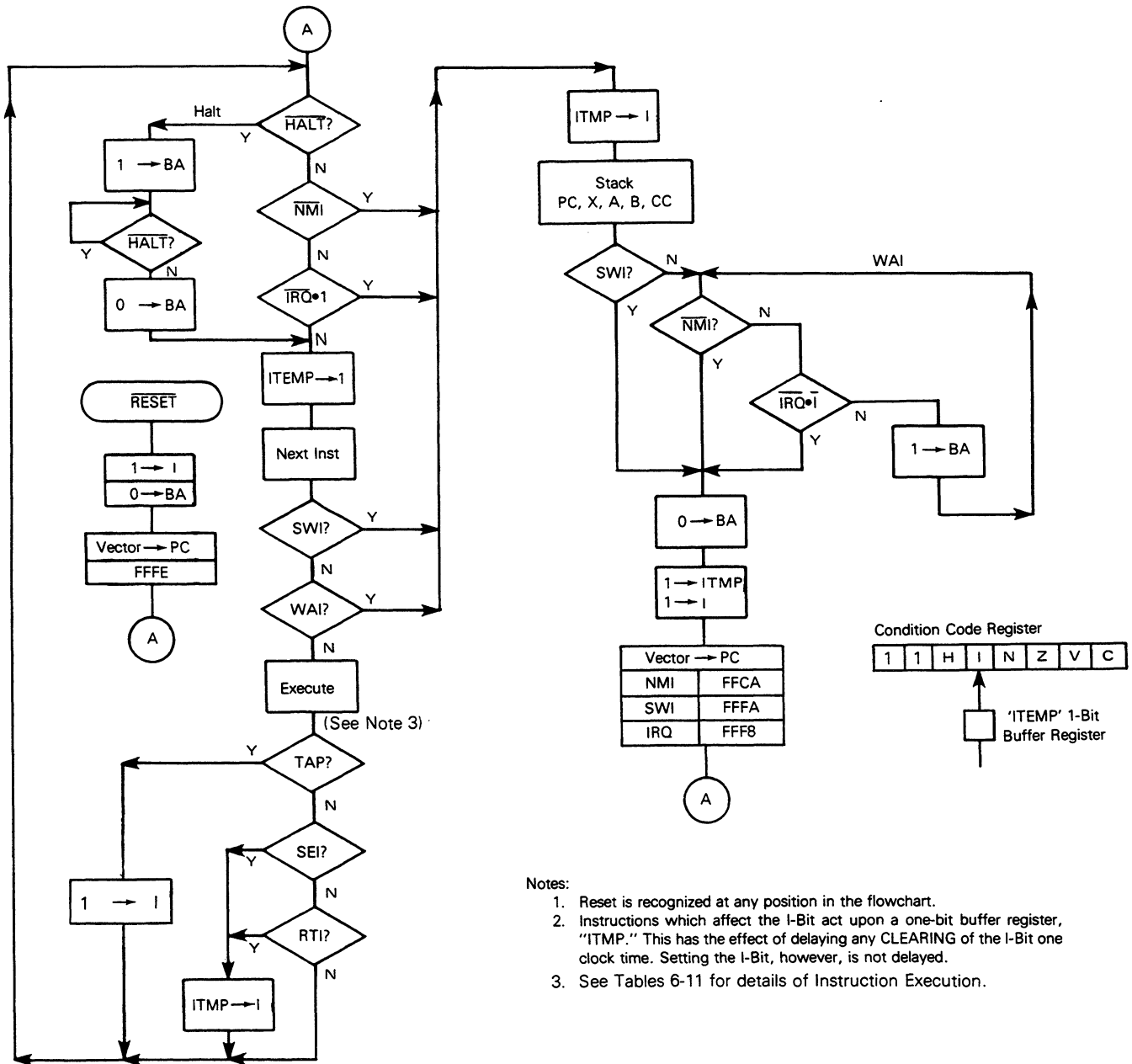
FIGURE 10 — MPU FLOWCHART
