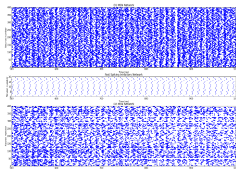
Figure 1. Raster plot of striatal microcircuit which comprises 400 D1 MSN (top), 20 FSIN (middle) and 400 D2 MSN (bottom).
