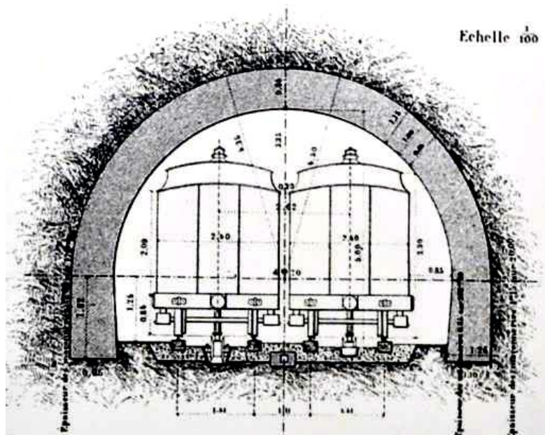
Figure 7. Sectional view of the tunnel (Gavand 1876)
