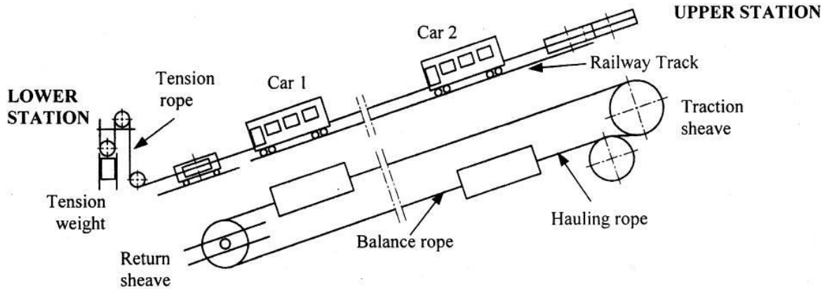
Figure 6. Overall configuration of Tünel (Imrak and Ozkirim 2002)
