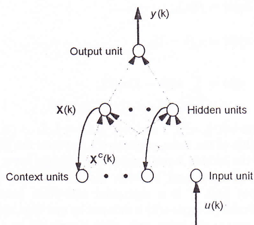
Figure 1. Basic Elman network.
