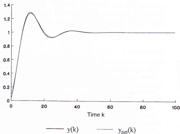
Figure 5. Response of modified Elman network with \alpha = 0.6 (second-order linear system).
