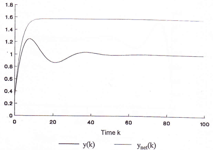
Figure 6. Response of Elman network trained by standard BP (third-order linear system).
