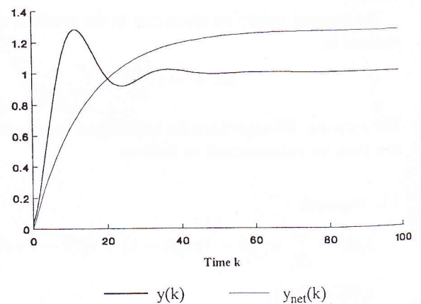
Figure 3. Response of Elman network trained by standard BP (second-order linear system).
