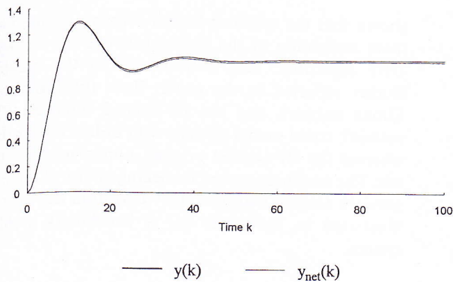
Figure 4. Response of Elman network trained by dynamic BP (second-order linear system).
