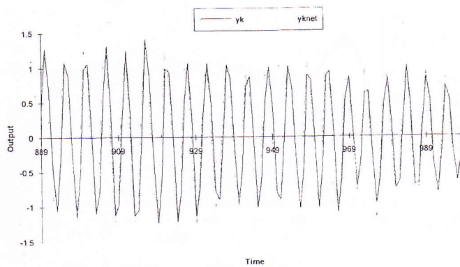
Figure 9. Response of nonlinear process (see (19)).
