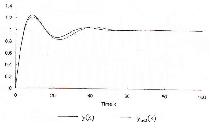
Figure 7. Response of Elman network trained by dynamic BP (third-order linear system).
