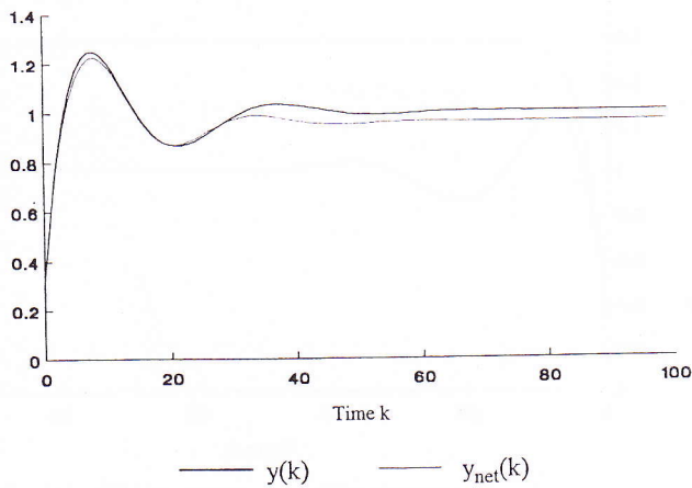
Figure 8. Response of modified Elman network with \alpha = 0.7 (third-order linear systems).
