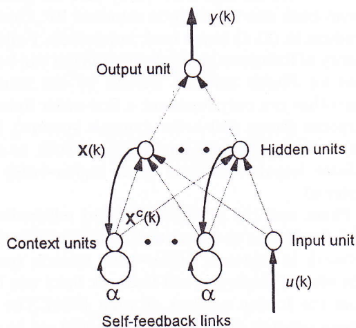
Figure 2. Modified Elman network.
