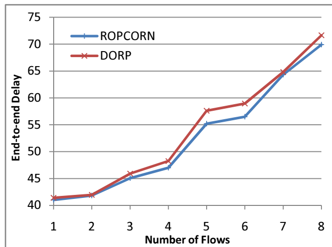
Figure 5. End-to-end delay performance compared to DORP
