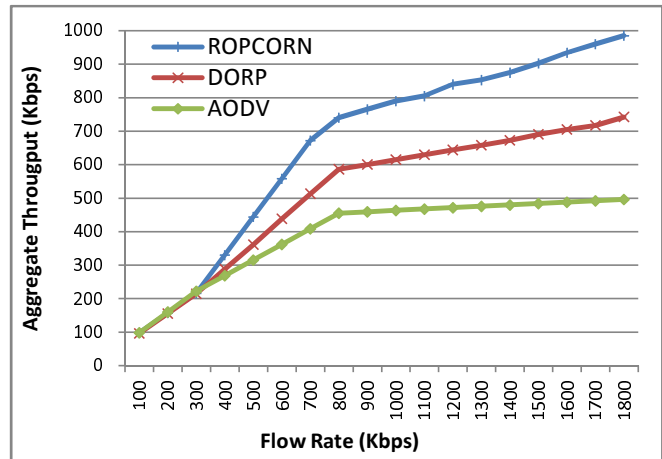
Figure 4. ROPCORN performance: throughput observed with different protocols
