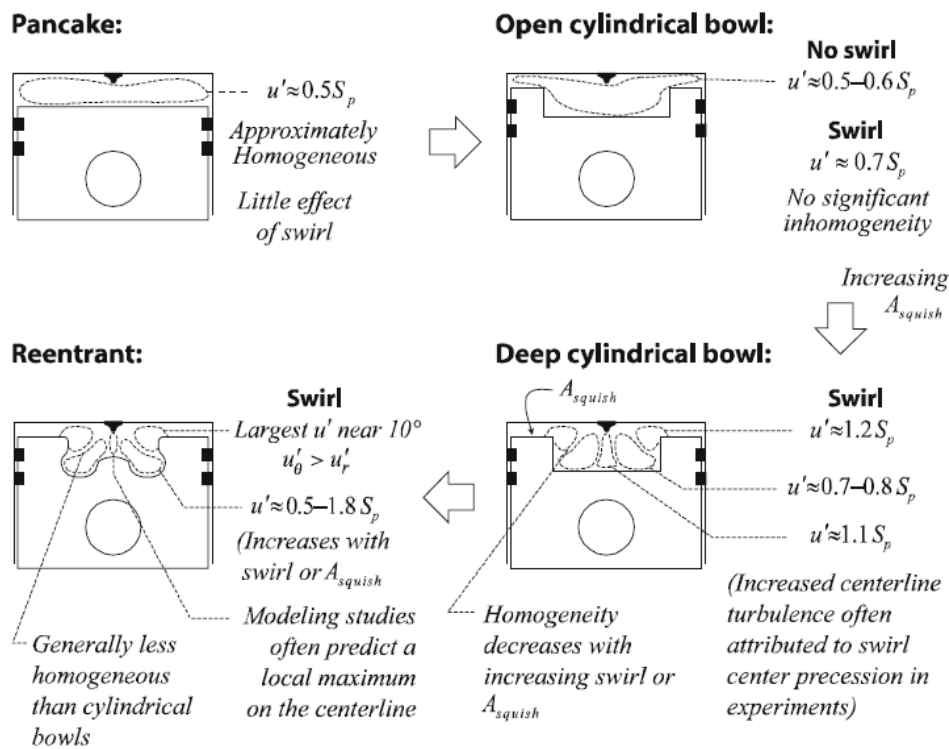
Figure 1. Swirl and squish effects for various piston types.
