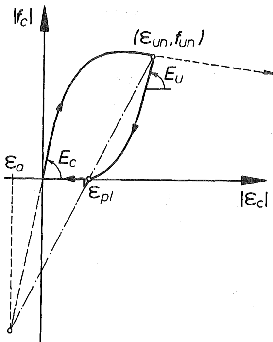
FIG. 5. Stress-Strain Curves for Unloading Branch and Determination of Plastic Strain \epsilon_{pl} from Common Strain \epsilon_a
